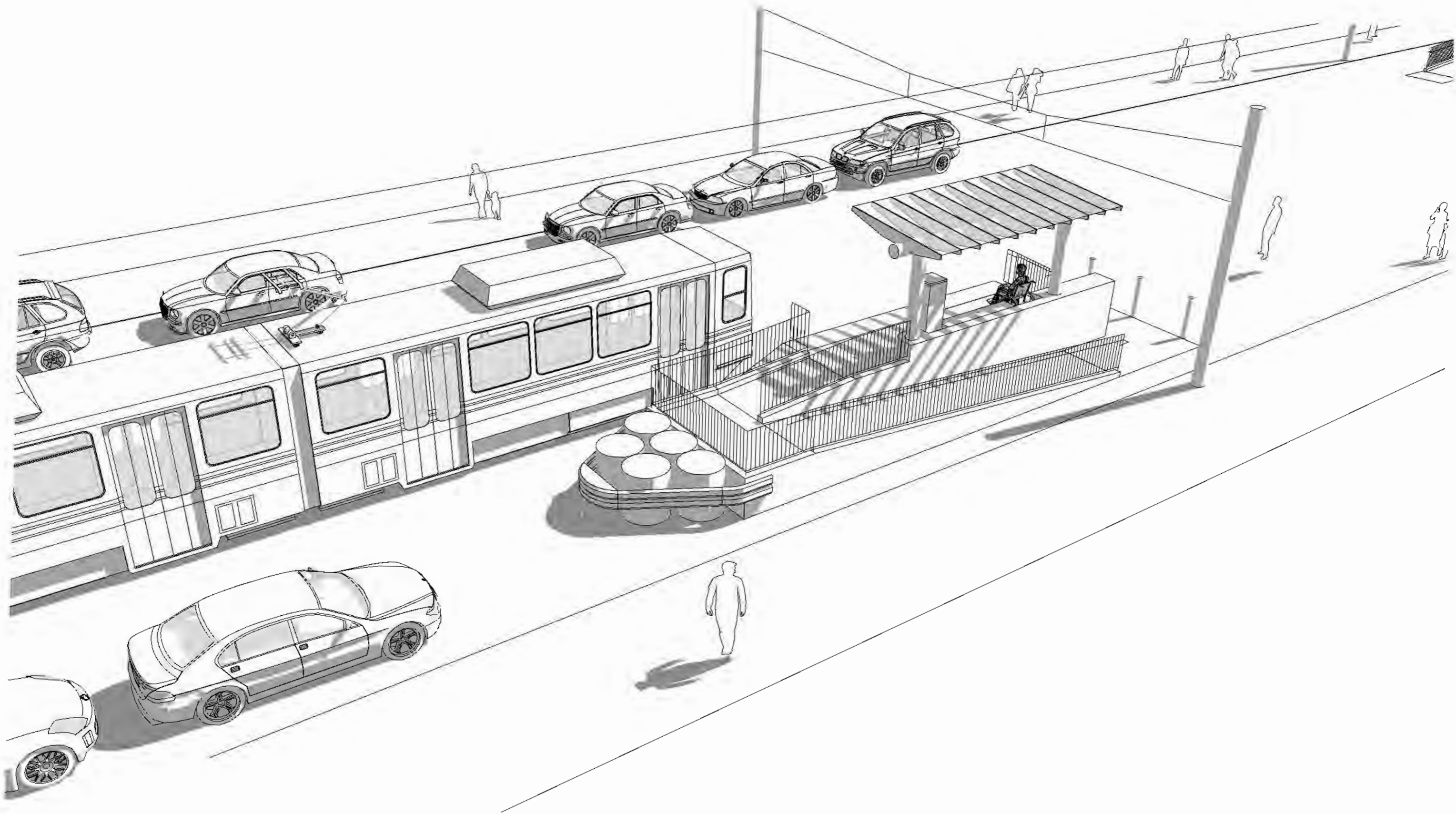
RAISED PLATFORM SWITCHBACK RAMP OVERALL VIEW
